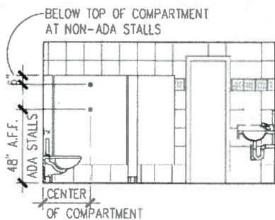
HEAVY DUTY COAT HOOKS AT RESTROOM PARTITIONS
